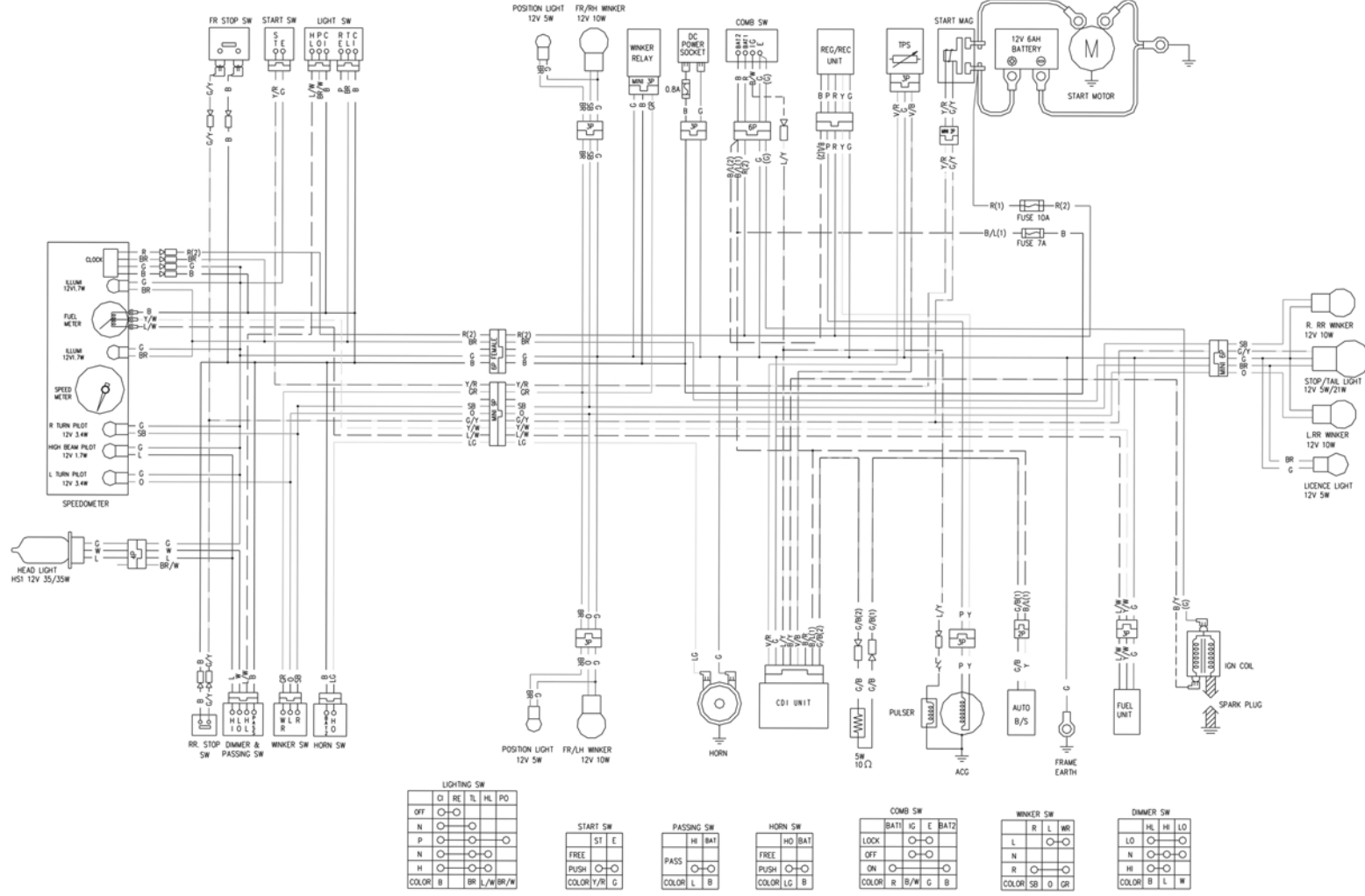
LIKE 50/125 WIRING DIAGRAM
